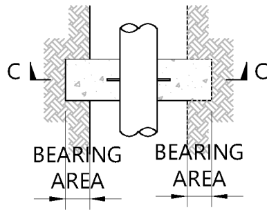
TYPICAL IN-LINE THRUST BLOCK DETAIL - PLAN VIEW
