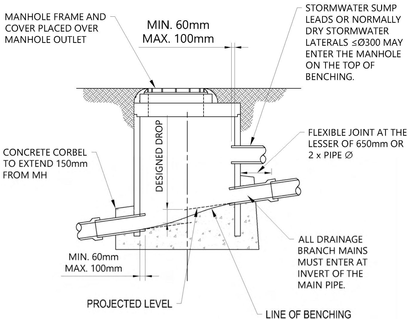
CROSS SECTION THROUGH STORMWATER MANHOLE
